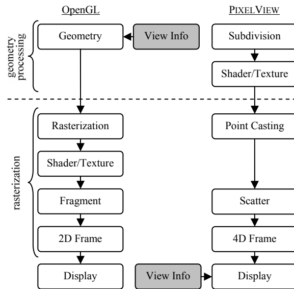
Figure 2: High-level comparison between a typical OpenGL-style pipeline and PixelView. Only the display stage in PixelView requires knowledge of the viewpoint, allowing reuse of shading and rendering calculations.
