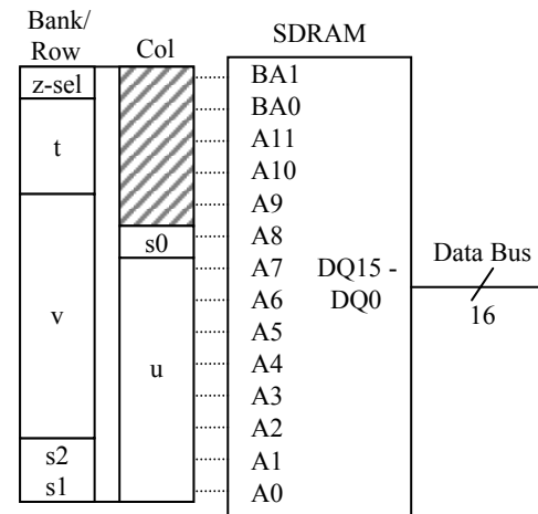
Figure 6: Swizzling of (s,t,u,v) samples into SDRAM addresses to achieve increased scan-out coherence. Half the banks are used for z-buffer data and half for color data, determined by the high order bank pin.
